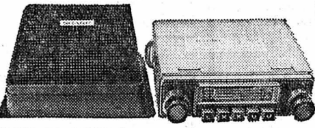
AR 942 Autoradio OUC/OM/OL/OC, 5 touches de station, 7 Watt, 160 x 50 x 130 mm Fr. 265.—
