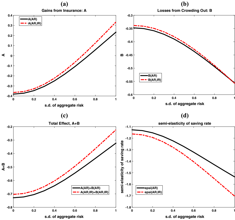
Fig. 1 Welfare effects in general equilibrium: high discount factor A and B are defined in proposition (4). Aggregate risk is AR = \sigma_Q^2 , because \sigma_\zeta does not enter in (4). A(AR) and B(AR) are for an economy with only aggregate risk, and A(AR, IR) and B(AR, IR) are for the economy with two separate risks
