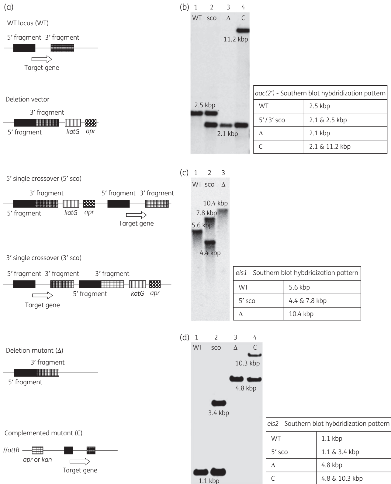
Figure 1. Genotypic analyses of M. abscessus deletion mutants. (a) General schematic drawing of genotypes and recombination events. (b) Southern blot analysis confirms the deletion of aac(2') ( MAB_4395 ) from the genome of M. abscessus . Genomic DNA of M. abscessus ATCC 19977 (lane 1), M. abscessus transformant with pSE- \Delta aac(2') targeting vector prior to (lane 2) and after KatG-dependent isoniazid counterselection (lane 3) and after transformation of counterselected mutant with pMV361- aac(2') complementation vector (lane 4) was digested with Van91I and probed with a
