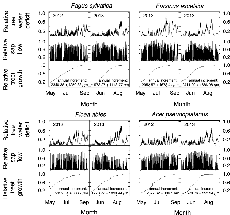
Figure 2. Relative tree water deficit, relative sap flow and relative tree growth during the growing season period (May 15 to September 30) for (a) P. abies ( n = 3 in 2012, n = 4 in 2013, SD_{rel \text{ tree water deficit}} = 0.17 , SD_{rel \text{ sap flow}} = 0.05 ), (b) F. excelsior ( n = 4 , SD_{rel \text{ tree water deficit}} = 0.12 , SD_{rel \text{ sap flow}} = 0.05 ), (c) F. sylvatica ( n = 4 , SD_{rel \text{ tree water deficit}} = 0.25 , SD_{rel \text{ sap flow}} = 0.04 ) and (d) A. pseudoplatanus ( n = 4 , SD_{rel \text{ tree water deficit}} = 0.18 , SD_{rel \text{ sap flow}} = 0.04 ). Tree water deficit, sap flow and tree growth were normalized for both years individually and are presented relative to the 2.5% yearly maximum values (see methods for details).
