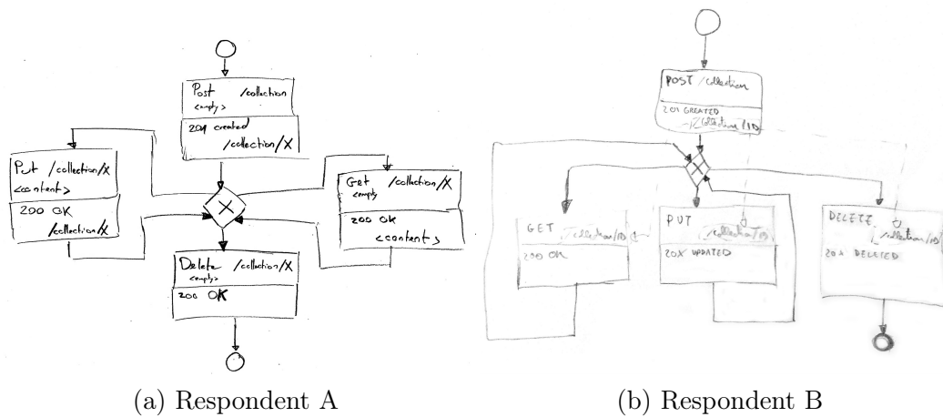
Figure 6.14. Respondents' models of CRUD operations on a collection item
