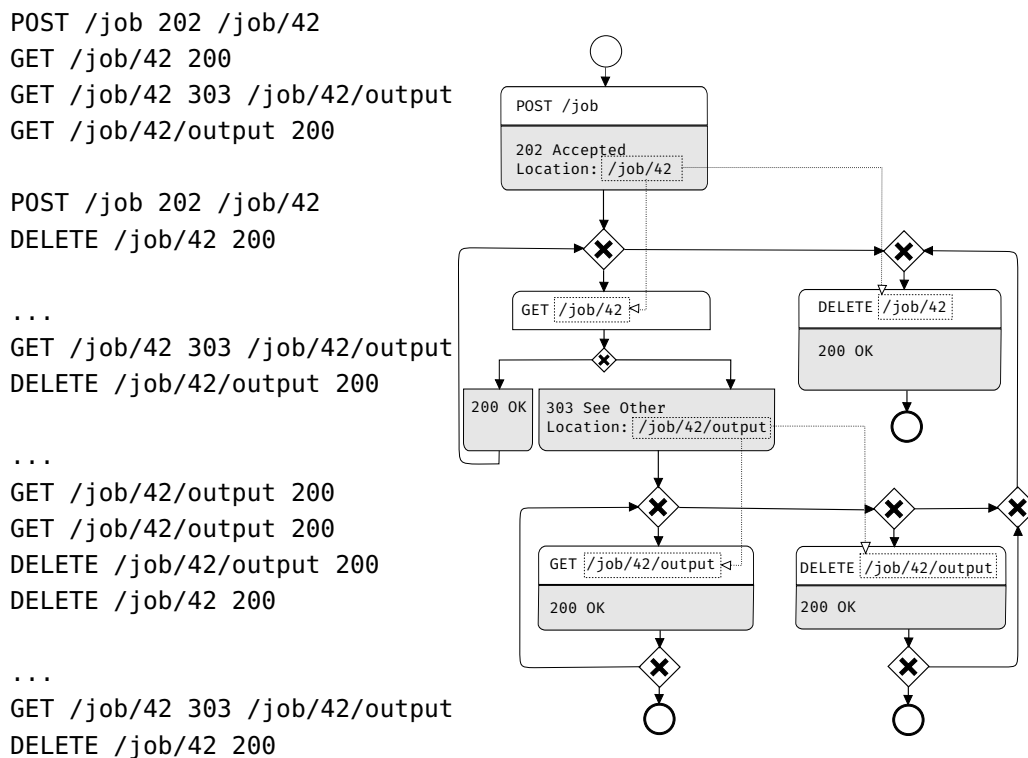
Figure 6.21. RESTalk textual and visual model of the Long Running Operation with Polling pattern [160]
