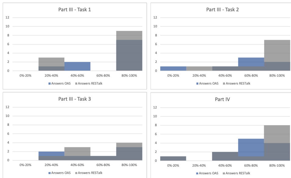
Figure 7.13. Distribution of Completion Time per availability of RESTalk diagrams in different tasks in Experiment 2
