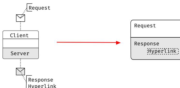
Figure 4.4. Modification 1: replacing the BPMN Choreography Task
