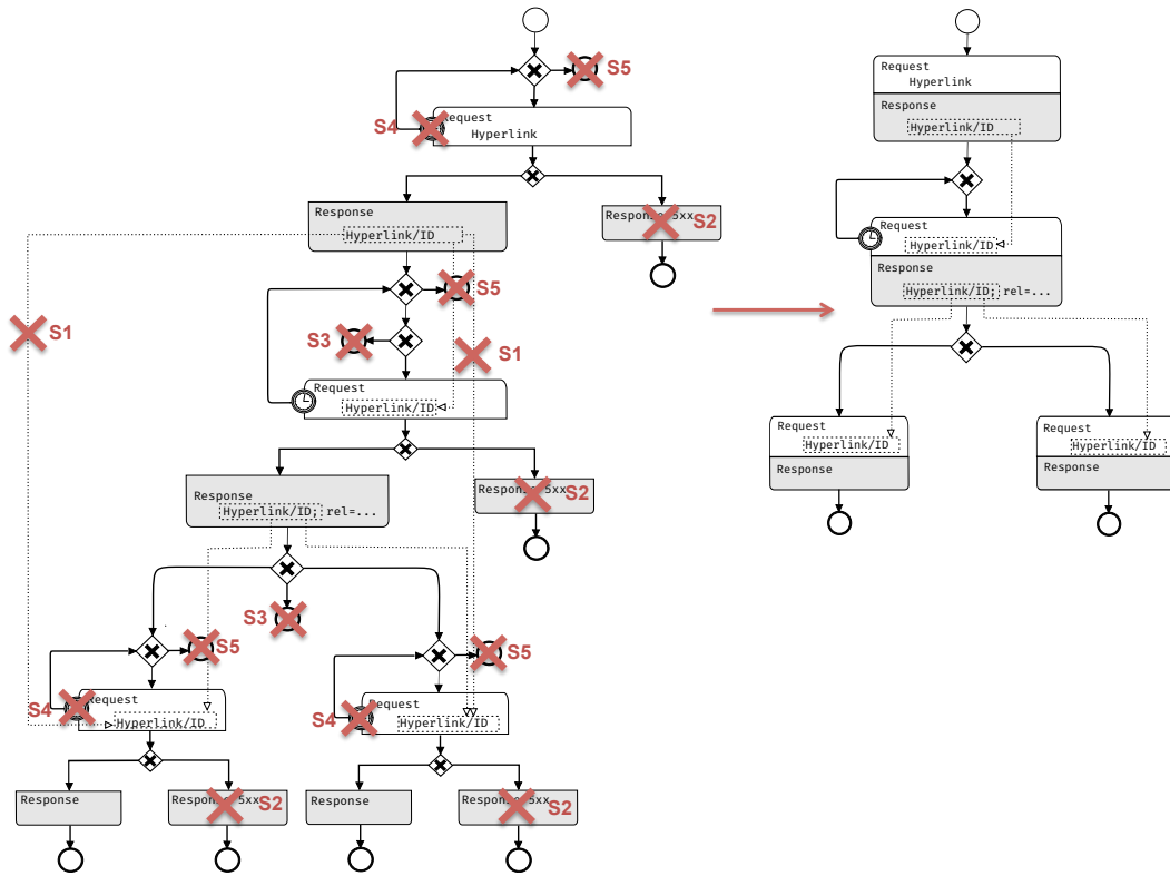
Figure 4.9. RESTalk diagram simplified following the simplification guidelines
