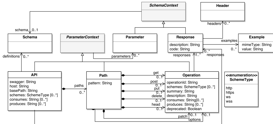
Figure 2.2. Behavioral elements of the OpenAPI metamodel
