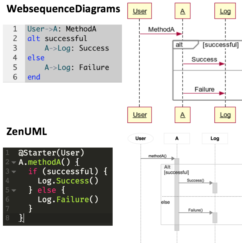
Figure 3.5. Sequence diagram definition in WebsequenceDiagrams vs ZenUML
