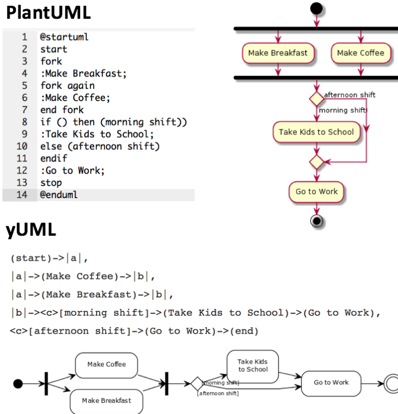
Figure 3.6. Activity diagram definition in PlantUML vs yUML
