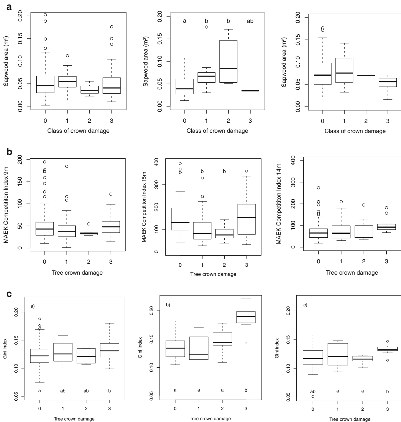
Fig. 5 Relationship between tree crown damage and sapwood area (a), the relative degree of competition experienced by these trees ( RCI_{\text{on\_stumps}} ; MAEK equation) (b), and the Gini index (c) on Mont
