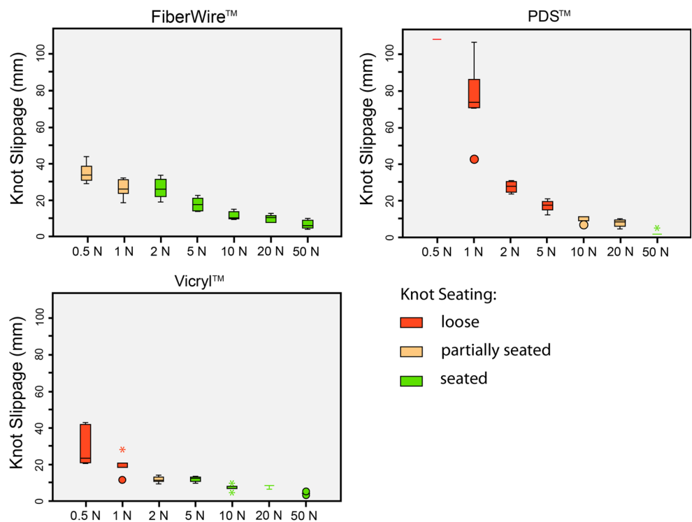
Fig. 8 Knot slippage related to used tying load (x axis) with colour-marked quality of knot seating
