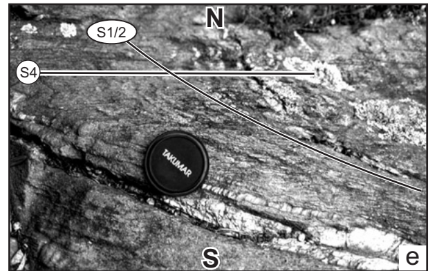
Fig. 8. D4 fold structures within paragneisses from the Camughera-Moncucco unit in Val Antrona. Figure 8a is from north of the axial plane of the Vanzone antiform; Figures 8b, c are from an outcrop situated south of the Vanzone axial plane; Figures 8d, e are situated south of Vanzone axial plane. Note the changing asymmetry of D4 folds across the hinge of the Vanzone antiform, while the sense of shear (Fig. 8a, c) remains the same.
