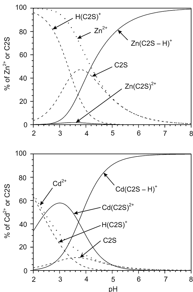
Fig. 3 Effect of pH on the concentrations of the species present in aqueous solution of the \text{Zn}^{2+}/\text{C2S} (top) and \text{Cd}^{2+}/\text{C2S} (bottom) systems. The results are given as the percentages of the total C2S or \text{M}^{2+} concentrations which are present in a 1:1 ratio (1 mM). The calculations were done with the equilibrium constants listed in Table 1 for a concentration of 10^{-3} M for each reactant (25 °C; I = 0.5 M, \text{KNO}_3 ) (for the concentrations employed in the experiments see “Materials and methods”). The broken lines indicate the free ligand species, the dotted lines free \text{M}^{2+} , and the solid lines the metal ion complexes. Note, the possible formation of hydroxo complexes (especially in the case of \text{Zn}^{2+} ) [36] in the uppermost pH range is not considered in the calculations. Furthermore, the concentration of (\text{C2S-H})^- is not seen in the figure because this species occurs only at high pH, i.e., outside the pH range shown
