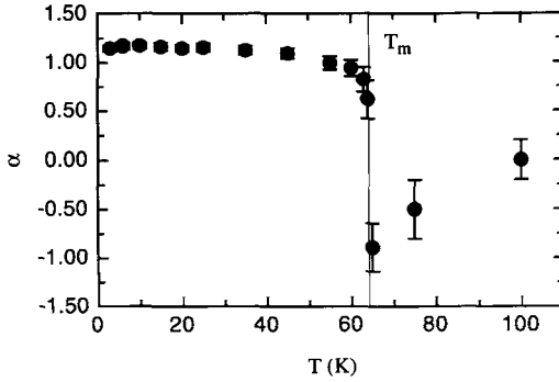
Fig. 6. The skewness of the \mu SR-lineshape may be represented by a quantity \alpha derived from the third and second moments of the probability distribution p(B) (see text). The lineshape and corresponding \alpha observed below the transition temperature T_m are characteristic of a vortex-line lattice, the disappearance of which is indicated by the sharp change of \alpha at T_m [7, 27]. These data are field cooled measurements for an applied field of 30 mT.
