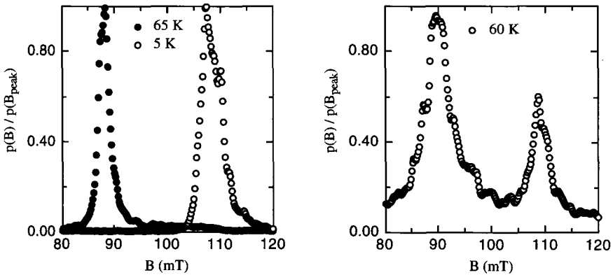
Fig. 9. The field distribution for a sample containing columnar defects at different temperatures. The spectra were taken after cooling the samples to 5 K in an applied field of 110 mT. The field was subsequently decreased to 90 mT and the sample temperature raised. For temperatures in the range of 55–60 K, the mean internal field changes from the value of the frozen field (110 mT) to the applied (90 mT). The value of the depinning temperature thus obtained is in good agreement with that obtained from magnetization measurements [47].
