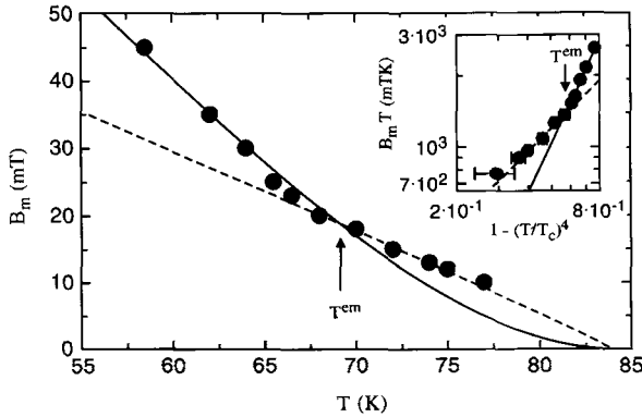
Fig. 7. Measurements taken from [27] of the phase line B_m(T) . This represents the transition of the vortex lattice in BSCCO as determined by changes in the \mu SR-lineshape, such as those represented in Fig. 6. Note the change in the curve at temperature T^{\text{em}} . The solid line is a fit of the data, for T < T^{\text{em}} , to the melting curve Eq. (1) of [27] with c_L = 0.18 , or alternatively a fit to the decoupling curve Eq. (4) of [27] with c_D = 0.076 . In this region, electromagnetic coupling between pancake vortices in adjacent superconducting layers is the dominant interaction. The dashed line is the decoupling function Eq. (3) of [27], with c_D taken from above, and a value of \gamma = 160 taken from the position of T^{\text{em}} (see text). The inset is a logarithmic plot of the data and fitted curves.
