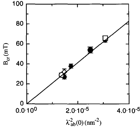
Fig. 4. The crossover field B_{cr} as a function of \lambda_{ab}^{-2}(0) for different samples of BSCCO. Open symbols correspond to \mu SR measurements on samples studied in [31]: circle is sample S_1 ; square S_2 ; diamond S_3 . Filled diamonds are taken from [34] and are obtained from magnetization measurement using Hall bar arrays. The filled circle is from a Tl-2212 sample taken from [35], where the crossover field is determined by magnetization measurements. The solid line corresponds to the relation B_{cr} = \Phi_0 / \lambda_{ab}^2 , which describes the data without any adjustable parameter.
