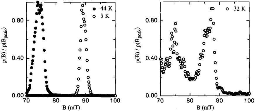
Fig. 8. Field distributions in BSCCO for different temperatures. The spectra were taken after cooling the samples to 5 K in an applied field of 90 mT. A field of 75 mT was subsequently applied. That the field distribution is not changed indicates strong pinning in this field and temperature range. As the temperature is raised, the mean internal field changes from 90 mT to 75 mT in the range 25–40 K. This reflects a thermal depinning of vortices and is in accord with the recent observation of a reemergence of Bragg peaks in SANS for the same temperature and field (Lloyd S.H., Aegerter C.M., Cubitt R., Lee S.L., Forgan E.M., Johnson S.T., Paul D.M c K., Wylie M.T., Nutley M.P., Kes P.H., Li T.W., unpubl.).
