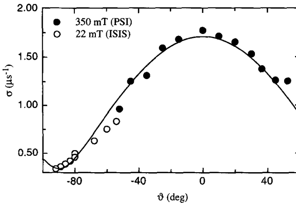
Fig. 2. The angular dependence of the \mu\text{SR} relaxation rate for a single-crystal sample of YBCO. As discussed in the text, the relaxation rate is assumed to be Gaussian, and is proportional to the second moment of the local field distribution. This quantity is a measure of the inverse square of the penetration depth and follows an angular dependence as given in Eq. (14). The solid line is a fit to this function resulting in a value of \gamma = 5 .
