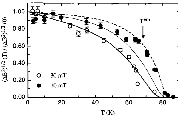
Fig. 3. Measurements taken from [26] of the \mu SR-linewidths \langle (\Delta B)^2 \rangle(B, T) in BSCCO at fields of 10 mT (filled circles) and 30 mT (empty circles). For T < T^{em} , T_m the data are described without any adjustable parameters by Eq. (15), using the appropriate expression for vortex fluctuations in this region, \langle u_{em}^2 \rangle^{1/2}(B, T) [28] (solid curves). The dashed line is the expected curve for T^{em} < T < T_m at 10 mT, using \langle u_{em,j}^2 \rangle(B, T) [28]. The 10 mT data migrates towards this curve for temperatures above T^{em} , reflecting the crossover illustrated in Fig. 7.
