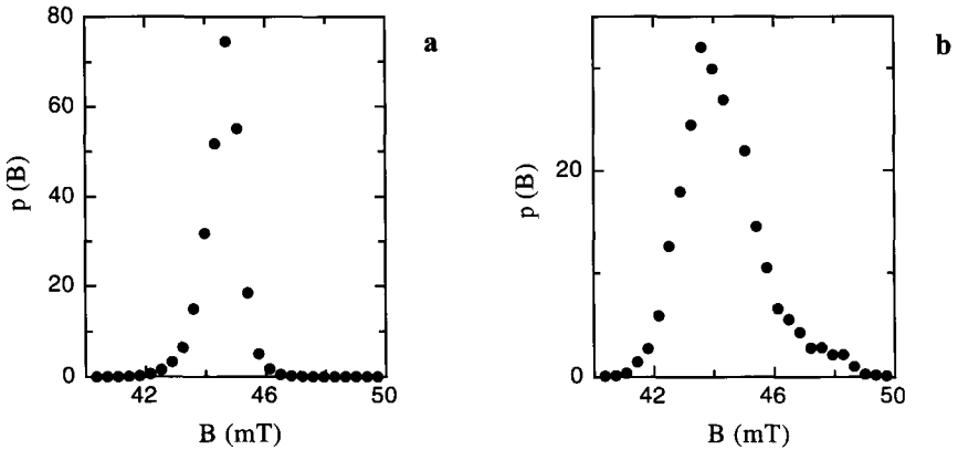
Fig. 5. \mu SR lineshapes for BSCCO in an applied field of 45 mT. a The line shape at 68 K, above the transition. b The line shape at 46 K, below the melting transition T_m .
