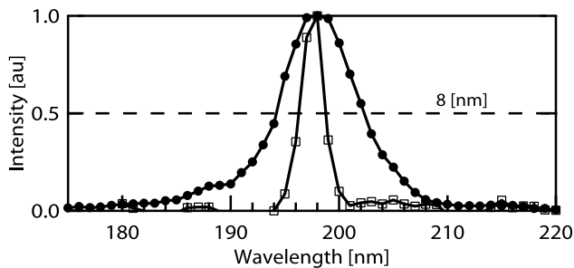
Fig. 4 UV spectrum (at 200 nm) of a B broad source obtained by co-filamentation ( dots ). Original spectrum corresponding traces for a 400 nm pulse without broadening ( squares ) (data reported from (Fig. 3(c)))
