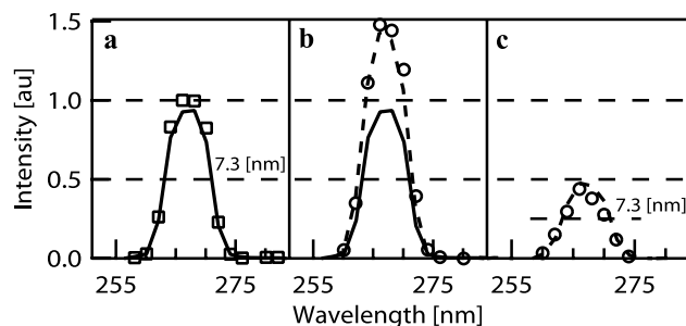
Fig. 5 Solid line : signal generated only by the IR beam. (a) Signal ( squares ) for UV and IR laser pulses temporally separated by 750 fs, (b) simultaneous and parallel ( dotted line ) (respectively perpendicular ( circles )) B and R laser pulses. (c) Signature of the SFG signal
