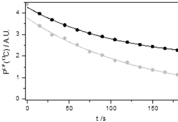
Fig. 8 Longitudinal ^{13}\text{C} relaxation in 3 M ^{13}\text{C} -labeled sodium acetate with 30 mM TEMPO in a 100 % deuterated water:ethanol (2:1 v/v) mixture after CP at 4.2 K and 3.35 T, either with 93.9 GHz microwave irradiation 'on' continuously (black dots) or switched 'off' after CP (gray dots)
