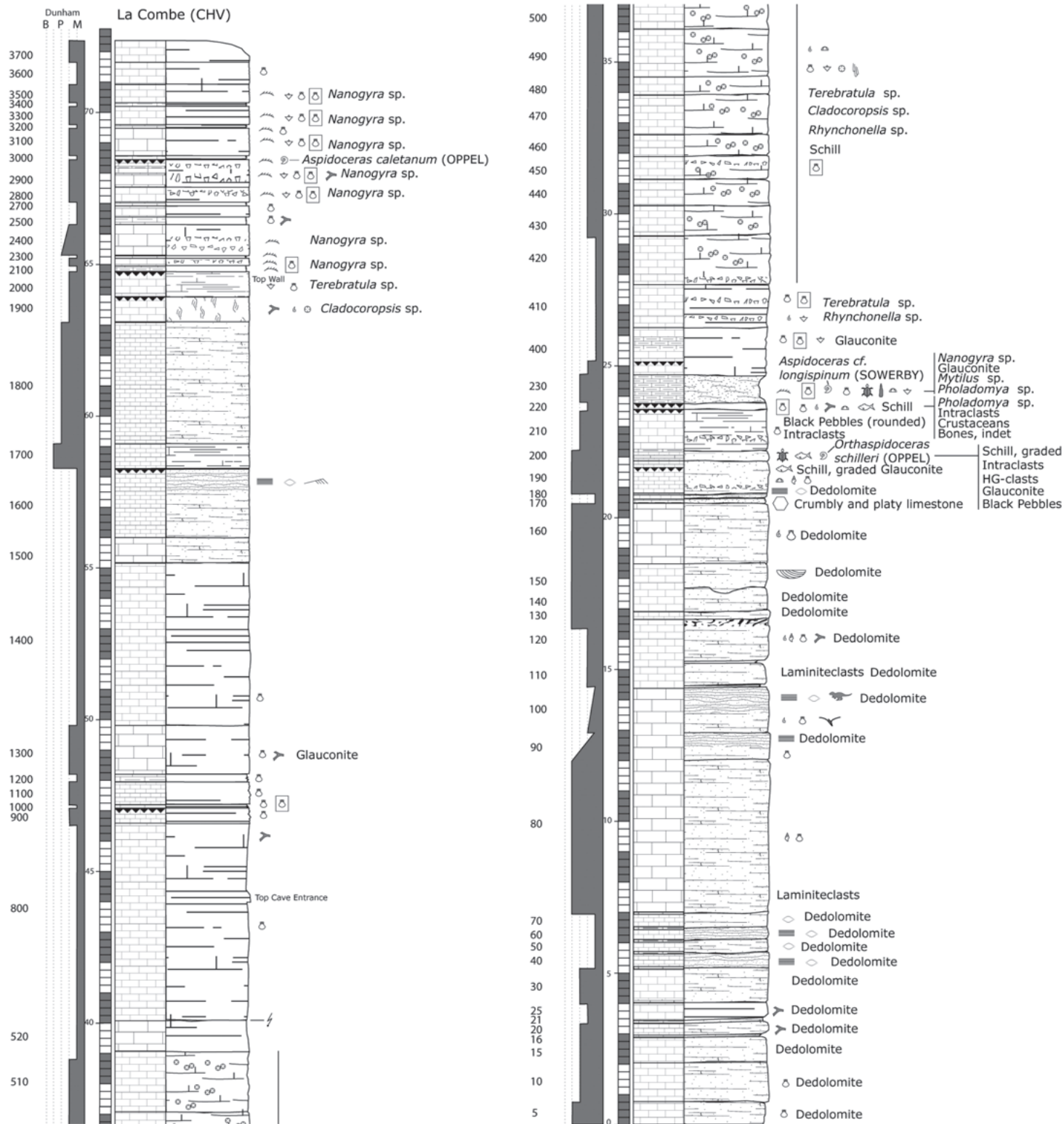
Fig. 5. Section La Combe – Bed CHV-230 are the Virgula Marls. For legend and symbols see Figs. 4 and 8.
