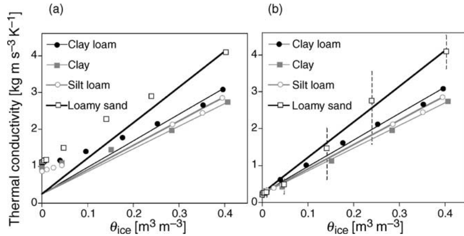
Figure 6. Thermal conductivities of prefractals generated according to the given particle-size distribution (symbols). The lines represent the calculations based on Johansen's approach. In one case (b) the heat transfer of particles is reduced. For the loamy sand, the range of calculated thermal conductivities is shown (dotted vertical lines).
