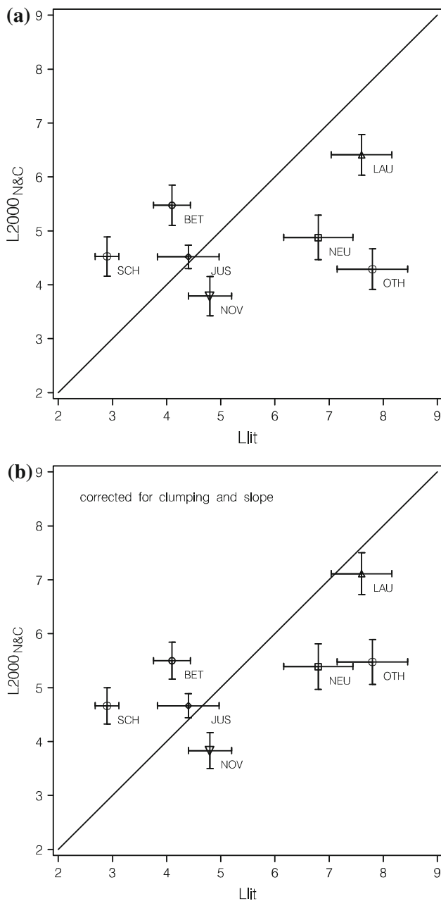
Fig. 7 Comparison of the litterfall and the LAI-2000 estimates (Norman and Campbell's equation). a Uncorrected L 2000 estimates. b L 2000 estimates corrected for clumping and slope. Bars indicate the standard errors
