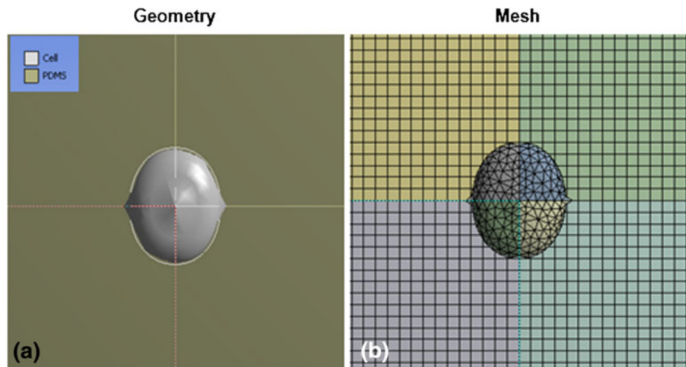
Fig. 1 (a) Geometry and (b) mesh of simplified representations of a cell on PDMS substrates, as modeled in the finite element analysis
