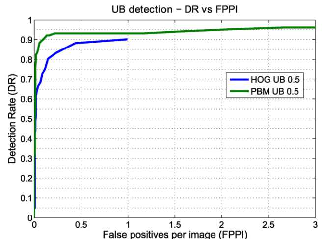
Fig. 9 Comparison of two frontal upper-body detectors: HOG (Dalal and Triggs 2005) and PBM (Felzenszwalb et al. 2008) . Test on Buffy video frames: 164 frames with 102 positive instances of frontal upper-bodies and 85 negative images. The curves correspond to a correct detection criterion of \text{IoU} > 0.5 . Detection rate is 0.9 at 0.1 FPPI (Color figure online)
