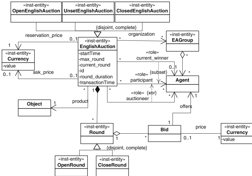
Fig. 3 Class diagram representing the english auction ontology
