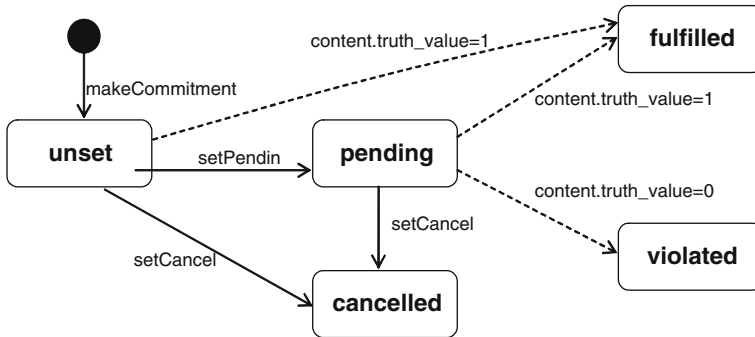
Fig. 2 The life-cycle of commitments
