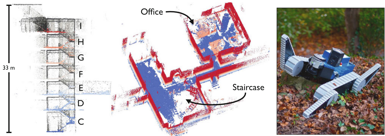
Fig. 4 Mapping of a seven-floor staircase using a search-and-rescue robot. Left Side view of the resulting map with the floor colored based on elevation. Middle Top view of the E floor with the ceiling removed and the points colored based on elevation. Right Photograph of the robot with climbing capability (Color figure online)
