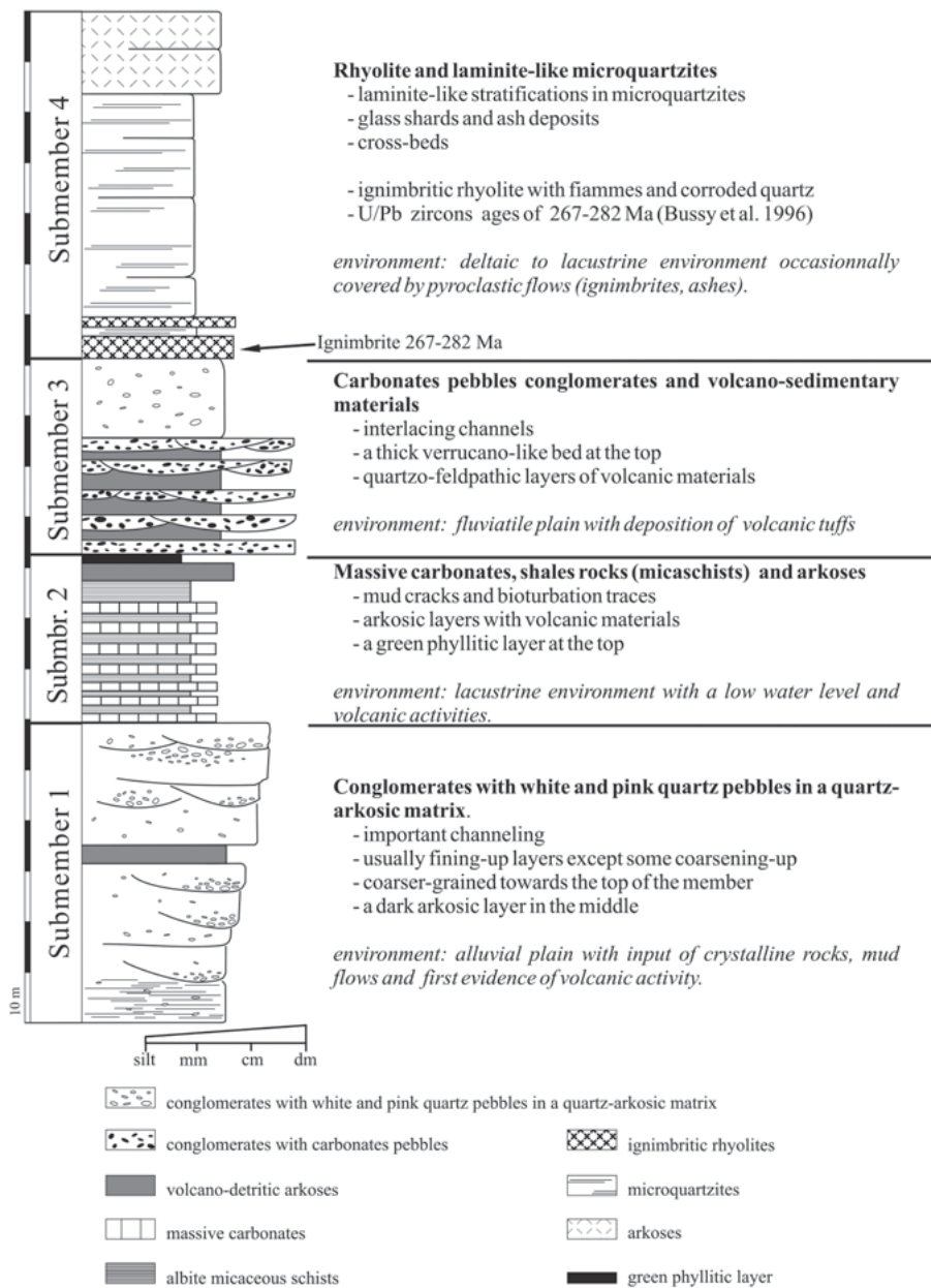
Fig. 3. Detailed stratigraphic log of the Goli d'Aget Member and interpretation of the environments of deposition. More accurate description of the lithology is in the text. The ignimbritic rhyolite lies at the bottom of the submember 4.
