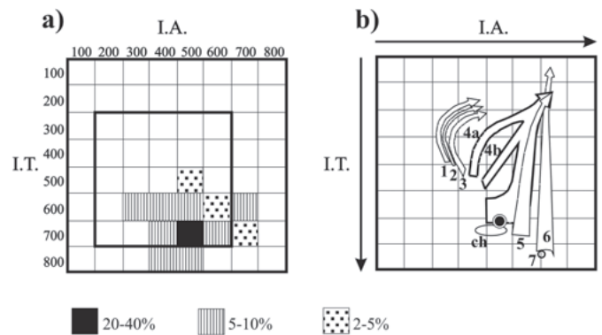
Fig. 4. Zircon typological diagram after Pupin (1980). a) Typological distribution of the Goli d'Aget rhyolite zircons in percent of zircons in each case, n=33. b) The white-rimmed black circle is the mean point (IA=494, IT=679) of the Goli d'Aget rhyolite zircons population. The different fields correspond to zircons from: (1) aluminous leucogranite, (2) (par)autochthonous monzogranites and granodiorites, (3) intrusive aluminous monzogranites and granodiorites, (4 a, b, c) calc-alkaline series granites, (5) sub-alkaline series granites, (6) alkaline series granites, (7) tholeiitic series granites, (ch) magmatic charnockites area.
