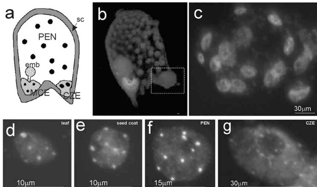
Fig. 1a–g Isolation of PEN and CZE nuclei. a Representation of the three endosperm domains in Arabidopsis : micropylar endosperm (MCE) surrounding the embryo (emb), peripheral endosperm (PEN), and chalazal endosperm (CZE). The maternal seed coat (sc) encapsulates the endosperm and embryo. b Seed at the globular embryo stage after digestion and dissection of the seed coat, as visualized by reflective light. The frame indicates the CZE. c The CZE remains as a multinucleate cyst after shearing the endosperm and spreading the nuclei on a slide; counterstained with DAPI. d–g Ethanol–acetic acid-fixed nuclei after spreading on a slide and counterstaining with DAPI (gray). Nuclei are from leaf ( d ), seed coat ( e ), PEN ( f ) and CZE ( g )
