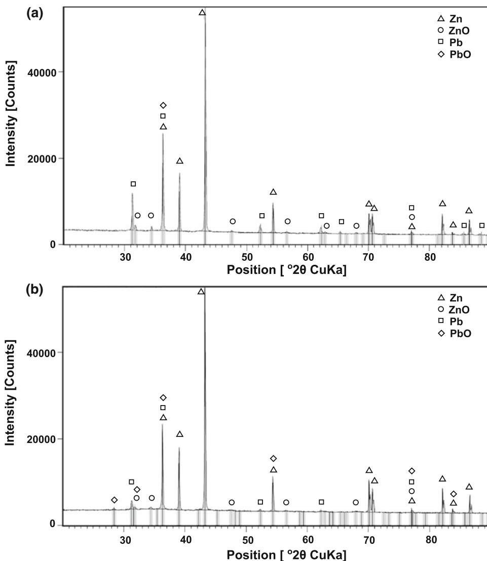
Fig. 13. XRD pattern of the condensed products for a representative run with (a) washed WOX (ZnO:C = 1:1.25, 1280°C) and (b) solar-clinkered WOX (30 min at T_{B1} = 1250°C, ZnO:C = 1:0.86, 1260°C).
