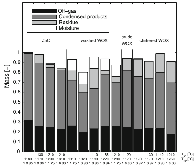
Fig. 12. Normalized mass balance of the solar carbothermal reduction experiments with different feedstock. The nominal temperatures at the bottom ( T_{B1} ) and top ( T_{B2} ) of the packed bed and the ZnO:C molar ratio are indicated in the x axis.
