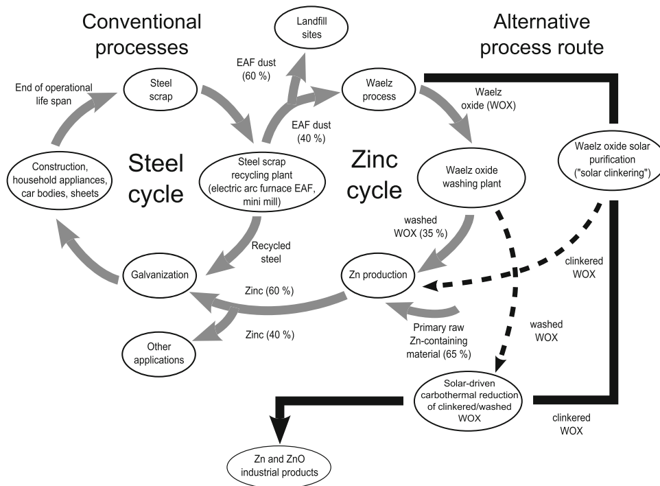
Fig. 1. Process flow diagram for the conventional steel and zinc industry and alternative routes using concentrated solar energy.
