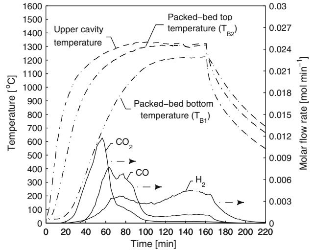
Fig. 5. Solar reactor temperatures and molar flow rates of CO, CO 2 , and H 2 during a representative solar clinkering experiment with 470 g of crude WOx.
