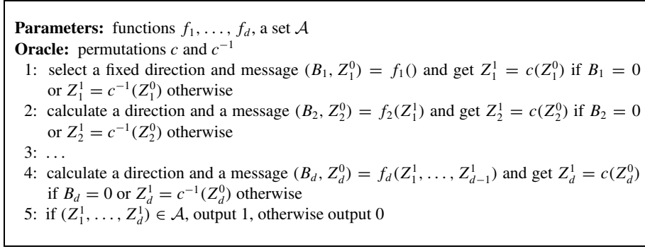
Fig. 8. A general d -limited distinguisher with chosen inputs or outputs.
