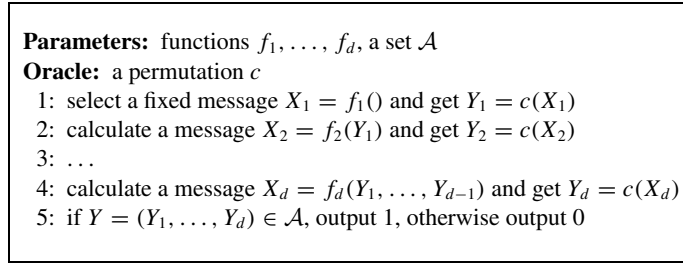
Fig. 1. A general d -limited distinguisher.
