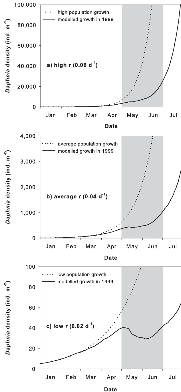
Figure 6a-c. Modelled spring population growth in Lake Brienz in 1999 with different growth rates (a-c). Dotted line: Modelled Daphnia density with average discharge and average temperature. Solid line: Modelled Daphnia density with elevated discharge and reduced water temperature of 1999. The grey shading shows the period of the flood. Note the different scales on the y-axes.
