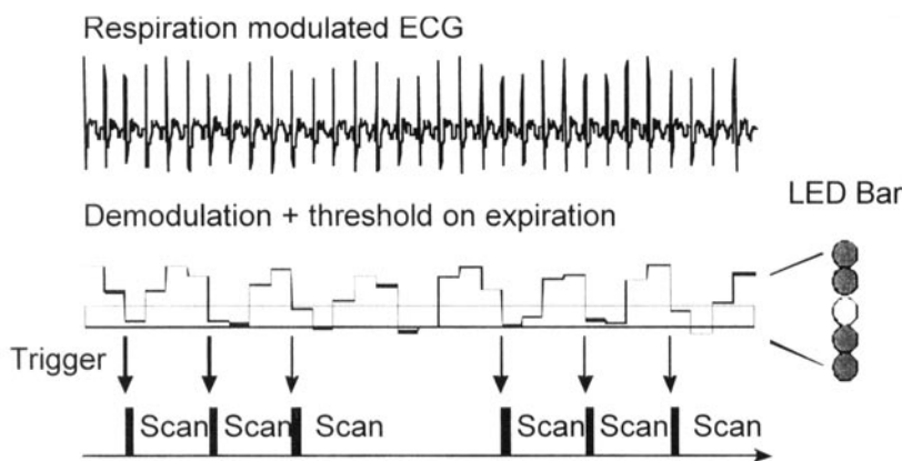
Fig. 2. Experimental scheme for combined respiratory/cardiac triggering based on respiration-related amplitude variations of the ECG signal (Scheme C).
