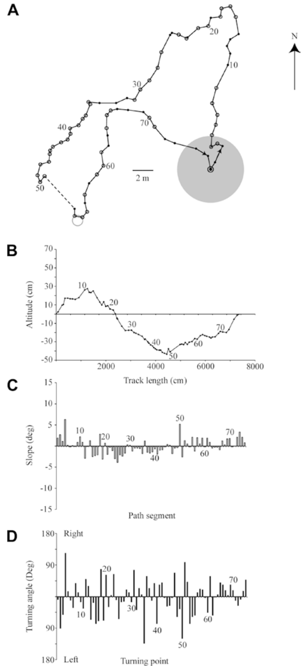
Fig. 1 A Example of a typical nocturnal path (projected on to the X - Y plane) of a male L. arenicola spider. The shaded grey circle represents the male spider's average territory size (average radius 3 m). The burrow (large black dot) is located at the centre of the depicted territory, and is surrounded by an area with a radius of 0.5 m (open circle) normally densely covered with the spider's footprints. The arrowheads indicate the direction in which the spider had walked. The small black dots mark the positions of the markers used in reconstructing the paths. The small circles along the path represent drum-marks made by the male. The large open circle shows the position of a mating track (approximately 1 m in diameter) around a female's burrow. The stippled line indicates where the spider crossed a harder stony surface, on which details of the path could not be recorded. B Altitude profile ( Z coordinate) of the spider's path. The burrow is positioned at the zero altitude line. C Histogram shows the degree of slope of each segment of the spider's path. D Histogram shows the size of the turning angle at each turning point along the spider's path
