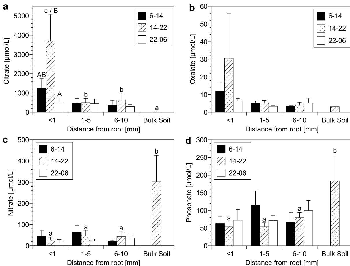
Fig. 4 Spatial and diurnal variation of citrate a , oxalate b , nitrate c and phosphate d concentrations in the rhizosphere of cluster roots of Lupinus albus during the time of maximum activity beginning on the 6–14 h sampling period before the first exudation peak and ending at the 22–6 h sampling period after the last exudation peak. Shown are the means and standard errors
