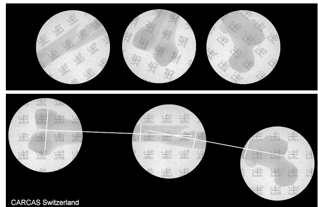
Figure 5. The individual fluoroscopy images (top panel) are scaled, de-rotated and positioned on the virtual grid in their true reciprocal position (lower panel). Subsequently guide lines can be drawn on the panorama images to visualize the fragment axis.
