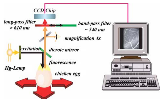
Fig. 2 Experimental set-up. Excitation was performed at 420 nm for verteporfin activation and 470 nm for FTIC fluorescence recording
