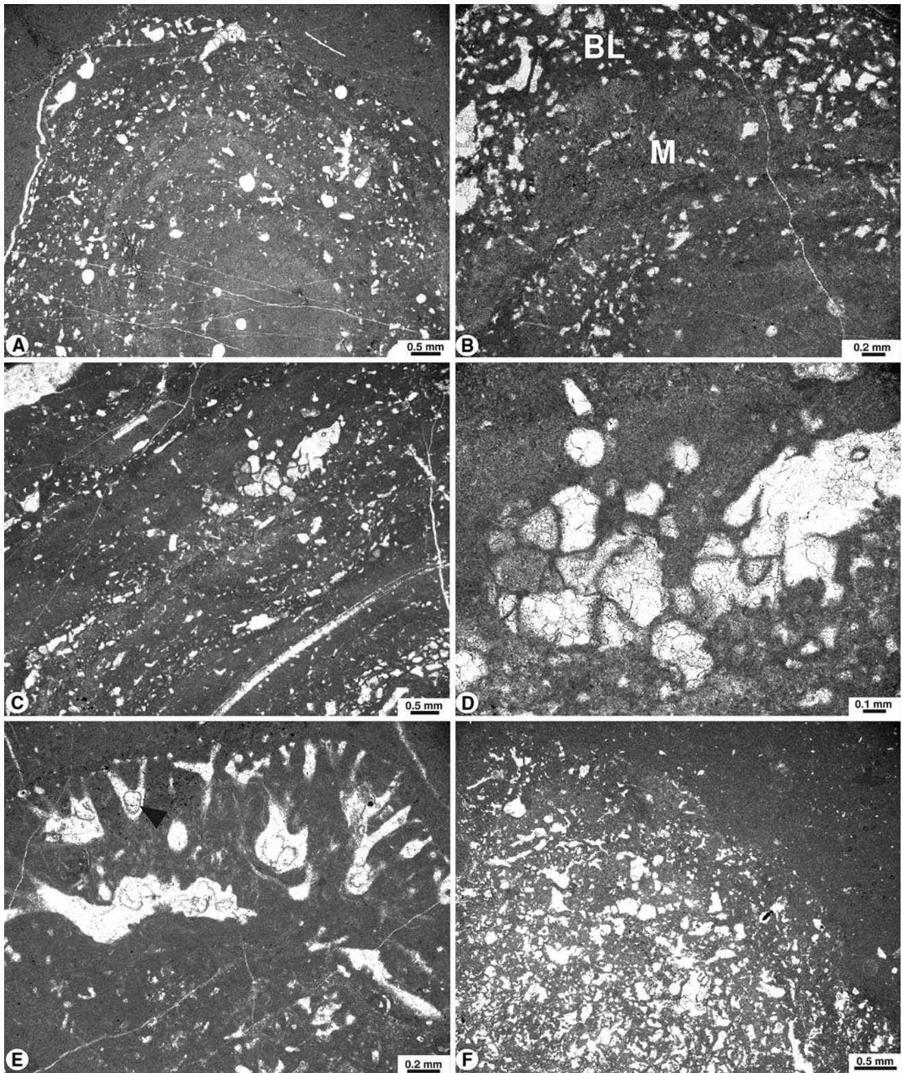
Fig. 10 Types 3 and 4 oncoids. a Type 3 oncooid with a cortex composed of irregular organism-bearing Bacinella – Lithocodium laminations and thinner micritic laminations. The contour is lobate. Pertuis section, thin section Pe-81A. b Detail of type 3 oncooid with Bacinella – Lithocodium meshwork BL and micritic laminations M. Pertuis section, thin section Pe-82A. c Detail of a type 3 oncooid cortex. Pertuis section, thin section Pe-82A. d Detail of the vesicular structure of
