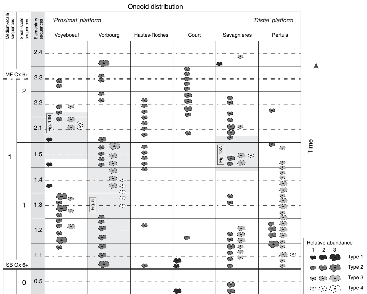
Fig. 12 Distribution of oncoïd types in the elementary sequences within the transgressive deposits of the Ox 6+ medium-scale sequence for the six studied sections. Sections are arranged from “proximal” to
