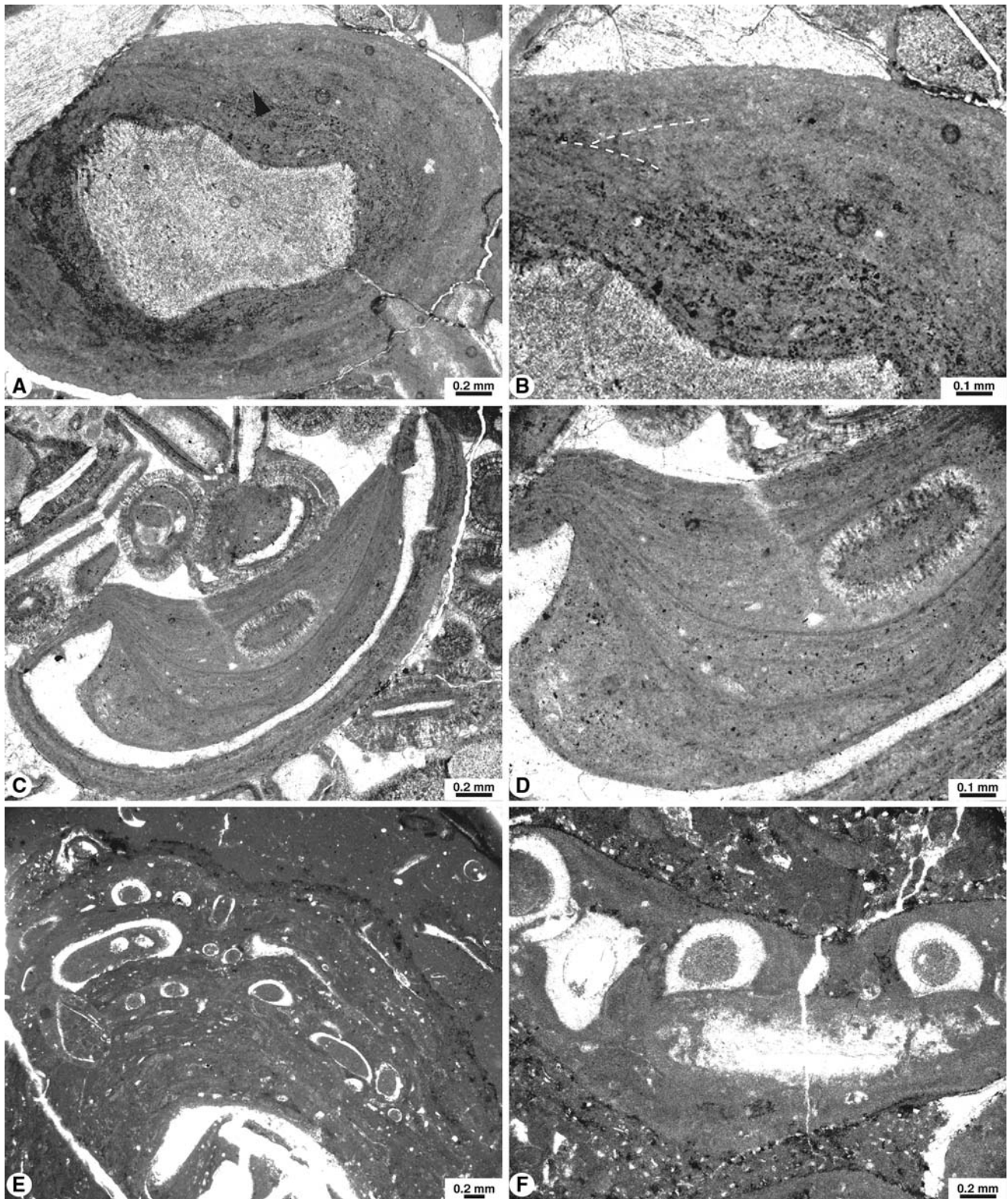
Fig. 9 Type 2 oncoids. a Elliptical oncoid with a large echinoderm fragment as nucleus and smooth contours. Micritic laminations of a first growth phase are onlapped by those of a second phase ( arrow ). Court section, thin section BPCo-81. b Detail of ( a ) showing the onlapping micritic laminae. Court section, thin section BPCo-81. c Elongate type 2 oncoid. In a first growth phase the laminae followed the shape of the nucleus. A radial ooid was then trapped, and in a second growth phase the cortex strived
