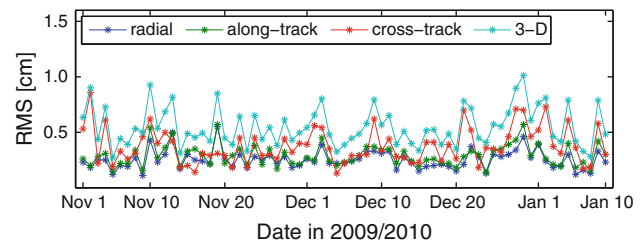
Fig. 11 RMS values (cm) for 5 h overlaps of RD PSO solutions
