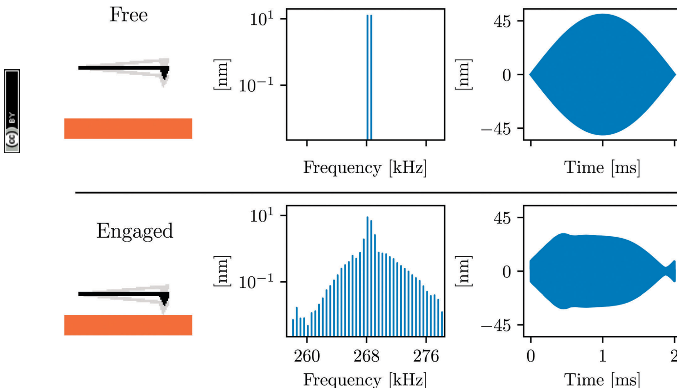
Fig. 1 Schematic illustrating the working principle of ImAFM: the cantilever is acoustically excited with two frequencies around its first flexural resonance. In the time domain, driving at two closely spaced frequencies gives a beating waveform, or slow modulation of a rapid oscillation. When engaging the sample surface many intermodulation products of the two drive tones are created around resonance, describing the distortion of the slow modulation. Conservative and dissipative force quadratures are reconstructed from the analysis of this distortion. 28–30
