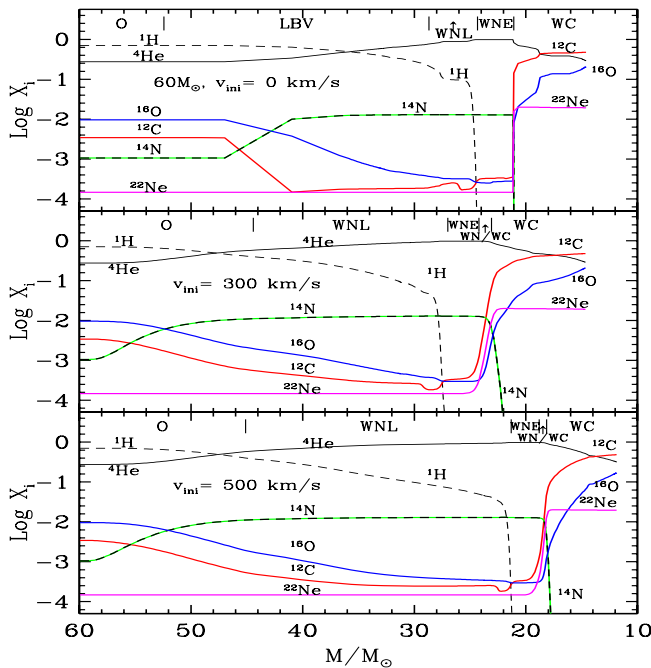
Figure 6. Evolution of the surface abundance for 60 M_{\odot} models at Z = 0.02 for 3 values of the initial velocities. From Meynet & Maeder (2003).
