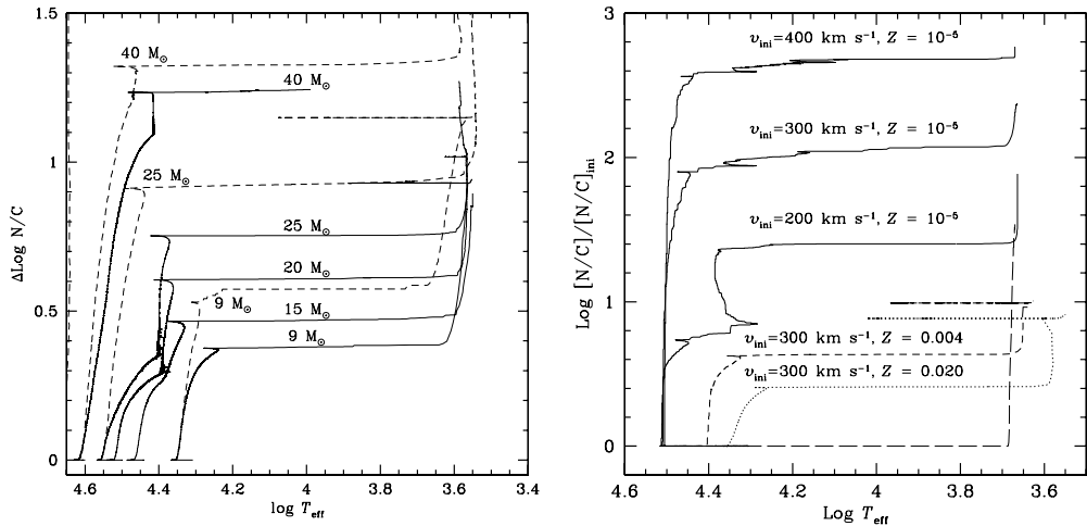
Figure 4. Left: evolution tracks in the plot \Delta \log(N/C) (change with respect to the initial N/C ratio) vs. \log T_{\text{eff}} for various initial masses with Z = 0.02 with initial velocities 300 \text{ km s}^{-1} (continuous lines). The dashed lines show the tracks with different model assumptions (Meynet & Maeder 2000). Right: excesses N/C in log scale for a 9 M_{\odot} star at different metallicities and rotation velocities. The long-dashed line, at the bottom, corresponds to a non-rotating 9 M_{\odot} stellar model at Z = 10^{-5} . From Meynet & Maeder (2002, 2003).
