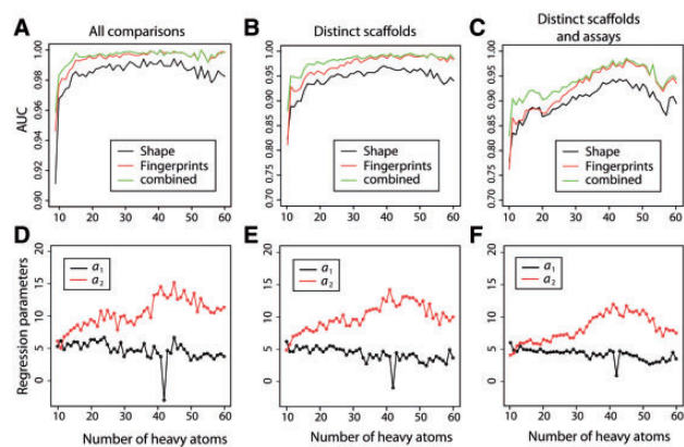
Fig. 4. AUC values for different molecule sizes. (A) The data obtained with the full ChEMBL dataset, (B) when restricting comparison to molecules with different scaffolds, and (C) when restricting comparison to molecules with different scaffolds and not tested in the same assays. Note the different y-axis scales. (D–F) regression coefficients for the combined approach
