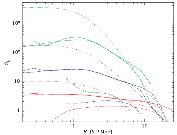
Figure 6. Hierarchical amplitudes S_k(R) for galaxy number count measured in numerical simulations for k = 3, 4 and 5 (bottom to top). Solid lines show galaxy (substructure) S_k , and long-dashed lines show halo S_{k,h} . Dotted lines show the point cluster model expressions in equations (30)–(32).
