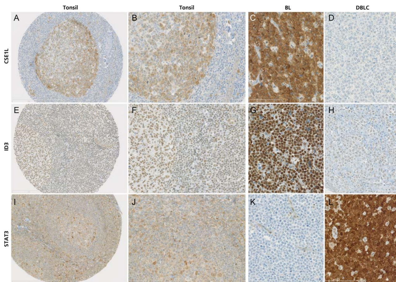
Figure 1. Results of immunohistochemical markers. 'CSE1L' in reactive lymphoid tissue at (A) low (20×) and (B) high power (40×) magnification with predominant, cytoplasmic reactivity in germinal-center dark cells and less strong in the light zone, but not in mantle zone cells or extra-follicular area. Examples (40×) of both (C) Burkitt's lymphoma (BL) and (D) diffuse large B-cell lymphoma (DLBCL). Inhibitor of DNA binding-3 (ID3) in reactive lymphoid tissue at (E) low and (F) high power magnification with nuclear reactivity in both germinal-center and mantle zone cells. Lymphoma examples of both (G) BL and (H) DLBCL. Signal transduction and transcription-3 (STAT3) in reactive lymphoid tissue at (I) low and (J) high power with only few cells with cytoplasmic reactivity, mainly in the extra-follicular area. Examples of samples of both (K) BL and (L) DLBCL.
