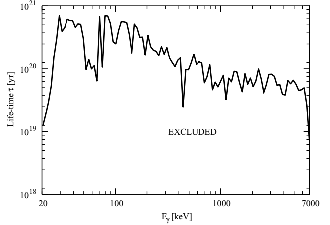
Figure 12. Lifetime of radiatively decaying DM as a function of the emitted photon energy. The region below the curve is excluded.
