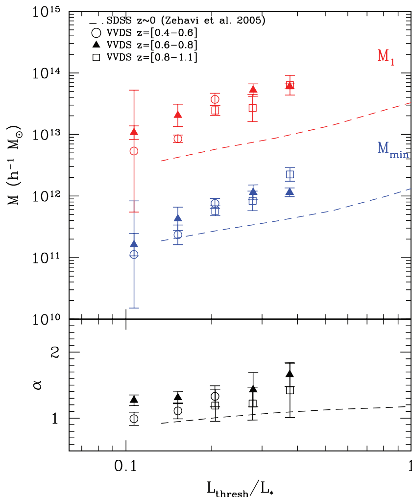
Figure 6. The best-fitting masses ( M_{\text{min}} , M_1 ) and power-law slope \alpha of haloes for Z model versus ( L_{\text{thresh}}/L_* ). The different symbols represent results for the VVDS, where each set of symbols correspond to samples lying in different redshift ranges (circles, solid triangles and empty squares represent samples having z = [0.4-0.6] , [0.6-0.8] , [0.8-1.1] , respectively). The superimposed dashed lines depict the SDSS.
