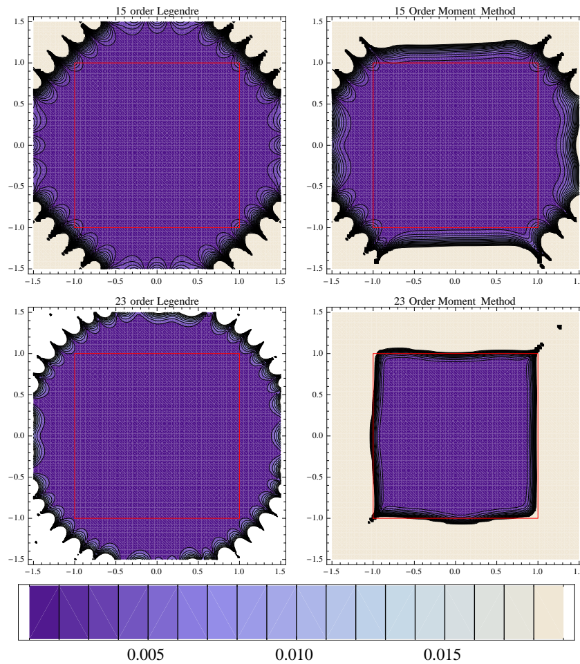
Figure 7: Comparison of the exact moment method on the right with the Legendre method on the left at 15 th and 23 rd order. These simulations used a uniform distribution with the red square denoting the region of integration. The potential was found both analytically using direct expansion around each point, and then it was determined using either the moment or Legendre methods to the indicated order, with the absolute difference indicated on the contour plot.
