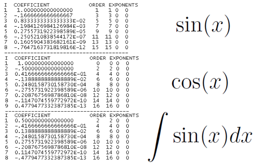
Figure 13: This shows examples of 16 th order one dimensional DA vectors for various functions. The expansions are around x=0 .
