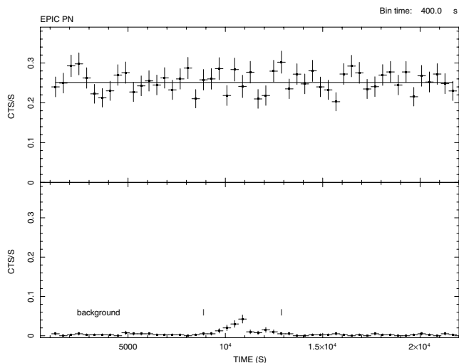
Figure 2. Background-subtracted EPIC pn light curve of WR 147 extracted from a circular region of radius 25 arcsec centred on WR 147 and binned at 400-s intervals (top panel). The energy range is 0.5–7 keV and the solid line is a constant count-rate fit to the data. Error bars are \pm 1\sigma . The bottom panel shows the background light curve extracted near the source in the 0.5–7 keV range. Vertical bars mark the high-background interval that was excluded from spectral analysis.
