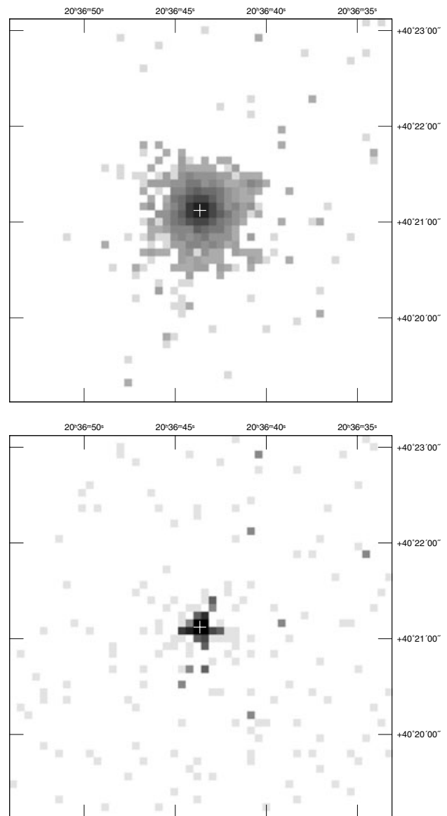
Figure 1. Top: EPIC pn image of the region near WR 147 in the 0.5–7 keV energy range on a log intensity scale, rebinned to a pixel size of 4.8 arcsec for display. Coordinates are J2000.0 and the cross marks the Simbad position of WR 147. Bottom: Same as above only restricted to the 6.3–7 keV range, dominated by Fe K\alpha emission.
