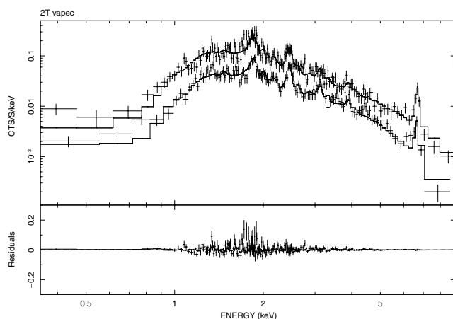
Figure 6. Best-fitting two-temperature optically thin plasma model 2T vapec (solid line) overlaid on the pn (top) and MOS1+2 spectra (bottom). Fit parameters are given in Table 1. Bottom panel shows fit residuals. Error bars are 1\sigma .
