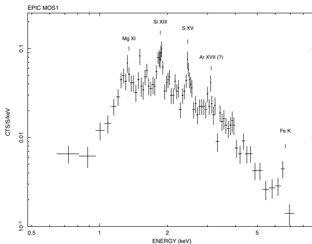
Figure 4. Background-subtracted time-filtered EPIC MOS1 spectrum of WR 147 (2085 net counts) extracted from a circular region of radius 25 arcsec and binned to a minimum of 20 counts per bin.
