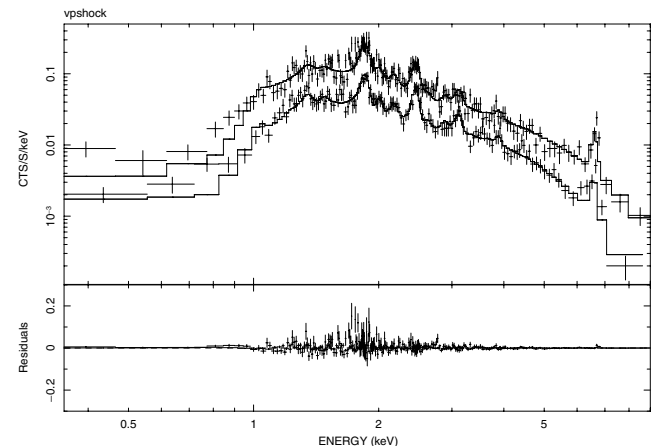
Figure 5. Best-fitting plane-parallel shock model vpshock (solid line) overlaid on the pn (top) and MOS1+2 spectra (bottom). Fit parameters are given in Table 1. Bottom panel shows fit residuals. Error bars are 1\sigma .
