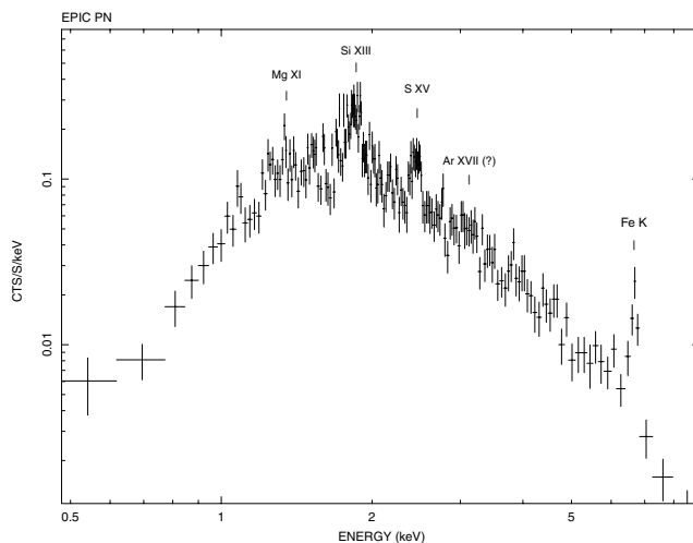
Figure 3. Background-subtracted time-filtered EPIC pn spectrum of WR 147 (4436 net counts) extracted from a circular region of radius 25 arcsec and binned to a minimum of 20 counts per bin.
