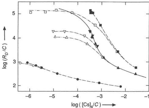
Fig. 7. Sorption behaviour of Cs-137 (open symbols) and of total cesium (filled symbols) in synthetic groundwater. ○● sorption on Montmorillonite; □■ sorption on Illite; △▲ sorption and ▽▼ desorption on a <32- \mu\text{m} fraction from Glattfelden with artificially increased content of exchangeable cesium.
