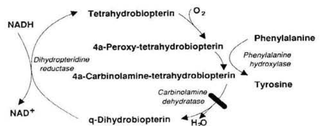
Figure 1. Phenylalanine-4-hydroxylase regenerating system and possible defect in primapterinuria.
