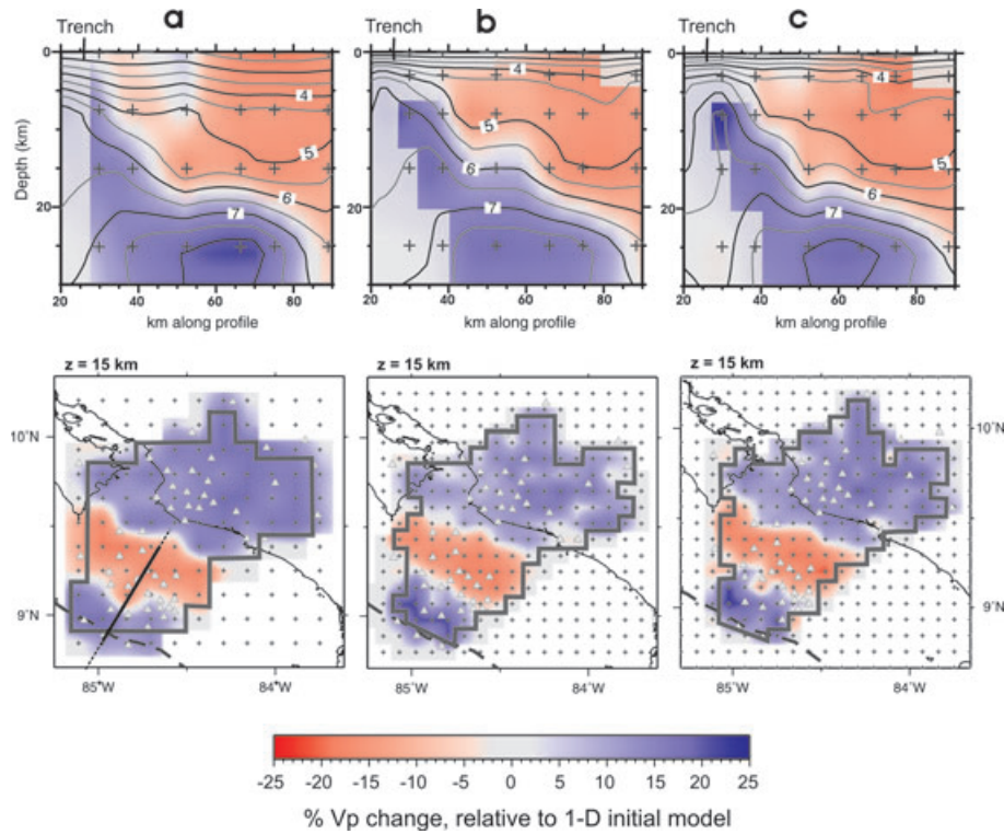
Figure 10. Effects of different model parametrizations on the tomographic image of Jacó seamount. Cross-section (as indicated) and depth slice from: (a) coarse horizontal grid of 15\text{ km} \times 15\text{ km} ; (b) horizontal grid 10\text{ km} \times 10\text{ km} , tuned vertical grid; (c) horizontal grid 10\text{ km} \times 10\text{ km} , tuned vertical grid and slight shifting of the coordinates origin of the horizontal grid. Grey lines encompass well-resolved areas as indicated by different resolution tests (see text for details). Triangles represent stations, and the dashed line the Middle America Trench. See text for discussion.
