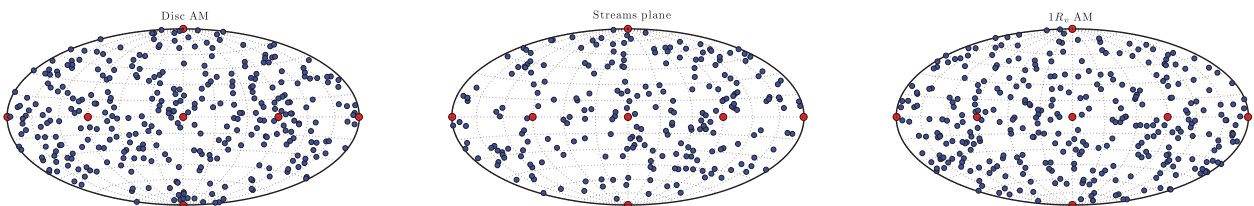
Figure C1. Numerical alignment. Hammer–Aitoff projection showing for each galaxy the direction of the normal to the plane in question (blue dots). The red dots represent the six directions of the simulation grid axes. Left: disc plane. Middle: SP at R_v . Right: AM at R_v . No obvious clustering of the blue dots about the red dots is noticeable, indicating that the numerical alignment with the simulation grid is weak.
