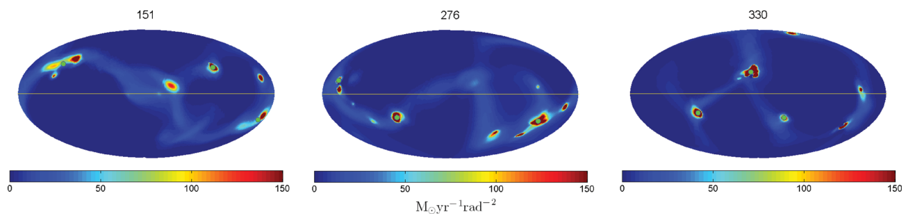
Figure D1. Poor SPs. Hammer–Aitoff projection for three haloes, similar to Fig. 3, showing the three worst cases for a SP.
