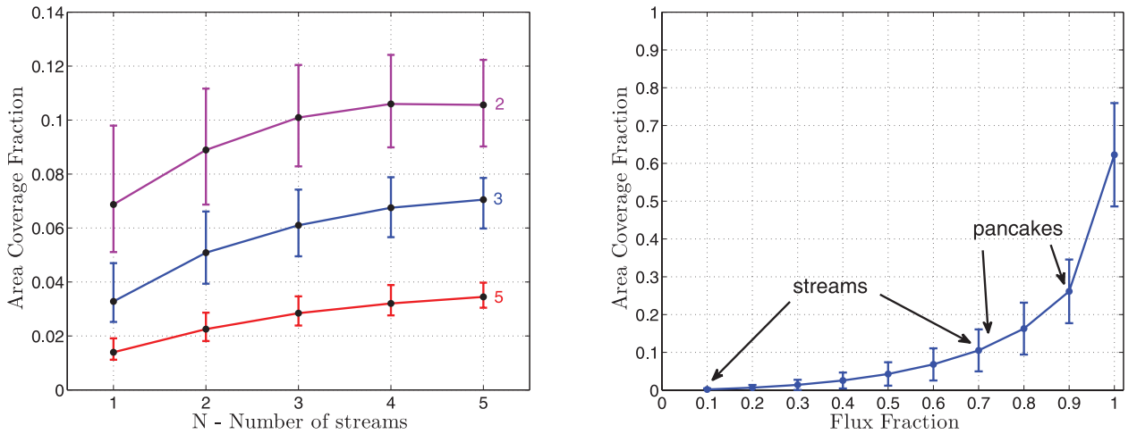
Figure 11. Fractional area coverage by streams and pancakes at R_v averaged over the 336 haloes. Left: area covered by the first N streams for flux overdensity thresholds 2, 3 and 5. With a threshold overdensity of 2, the first three streams have an averaging covering fraction of 10 per cent. Right: area coverage as a function of the corresponding fractional influx. The threshold of influx overdensity is varying along the curve, from \gg 1 to 2 for streams, and from 2 to 0.5 for pancakes. The streams carry on average about 70 per cent of the influx and cover 10 per cent of the angular area. The pancakes bring in about 20 per cent of the influx in 20 per cent of the area.
