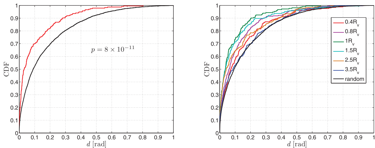
Figure 4. The significance of the stream coplanarity in a shell (1-2)R_v (left) and in shells of different radii (right). Shown is the cumulative probability distribution (CDF) of the rms deviation of the three largest streams from the best-fitting plane, d , based on 235 haloes (colour). It is compared to the same CDF for the null hypothesis of a random angular distribution of three points, based on 5000 realizations (black). The same threshold s_{\min} is applied to the data and the null model. A KS test reveals that at R_v the null hypothesis is strongly rejected with a p value of 8 \times 10^{-11} . The corresponding p values for shells from 0.4R_v to 3.5R_v are 0.12, 7 \times 10^{-5} , 2 \times 10^{-12} , 2 \times 10^{-8} , 4 \times 10^{-6} and 0.38.
