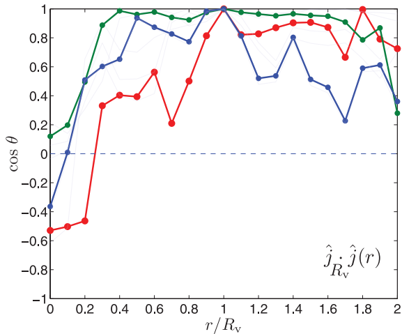
Figure 17. Three realizations from the distribution shown in Fig. 16 (right) of the alignment between the AM at R_v and in shells of other radii, displaying different behaviours. The green line (galaxy 250) shows a strong alignment from r = 1.9R_v down to 0.3R_v , followed by a drop in \cos(\theta) inside this radius toward zero. The red line (66) shows an alignment outside R_v and a change in direction immediately inside R_v leading to a slight anti-alignment inside 0.25R_v . The blue line (219) is an intermediate case, qualitatively similar to the median shown in Fig. 16.
