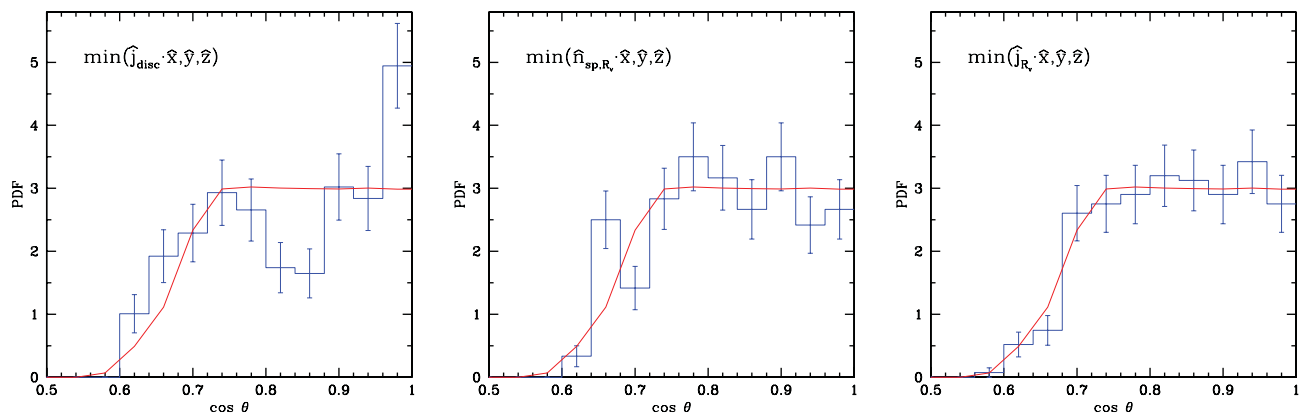
Figure C2. Numerical alignment. The distribution of the cosine of the angle between the normal to the plane in question and the closest simulation grid axis (blue). It is compared to the corresponding distribution for random plane orientations (red). Left: disc plane. Middle: SP at R_v . Right: AM at R_v . The disc shows a weak numerical alignment signal involving \sim 20 per cent of the discs at the level of \Delta \cos \theta \sim 0.08 .
