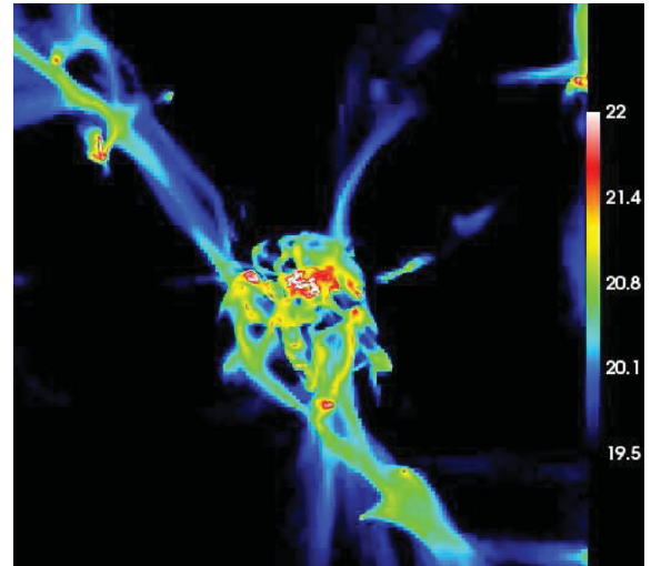
Figure 18. Surface density of cold gas in a galaxy simulated with 70-pc resolution (Ceverino et al. 2010). Beyond the coherent incoming streams coming from more than 100 kpc away, and the inner disc of radius \sim 6 kpc (white), there is a ‘messy’ region of radius \sim 20 kpc in which the perturbed distribution of matter results in strong torques and AM exchange – the AM sphere.
