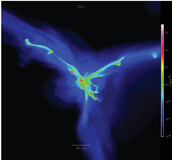
Figure 2. Gas density in the streams feeding the galaxy shown in the right-hand panel of Fig. 1 (314), in a RAMSES test run with a resolution higher by an order of magnitude. The box encompasses a sphere of twice the virial radius. The stream configuration remains qualitatively similar, with the inner structure of the streams better resolved (courtesy of D. Tweed).
