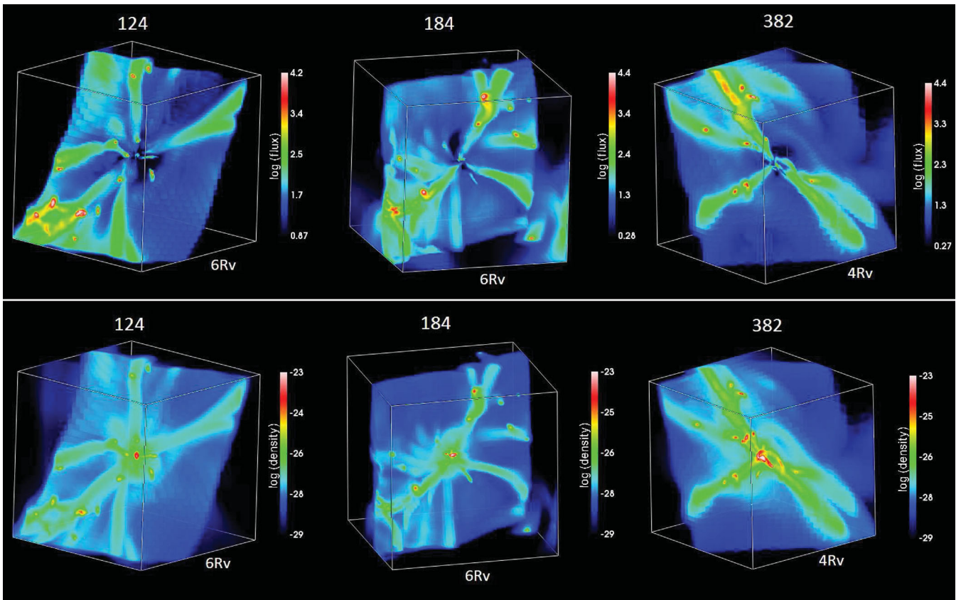
Figure 7. Cold streams embedded in pancakes, flowing into three different simulated galaxies. The box side is marked in each case. No temperature threshold is applied. Top: log influx density (in M_\odot \text{ yr}^{-1} \text{ rad}^{-2} ). Bottom: log gas density (in \text{g cm}^{-3} ). The planar pancakes and elongated streams become apparent in this ray-casting maximum-intensity projection, which shows the maximum intensity volumetric pixel along the line of sight.
