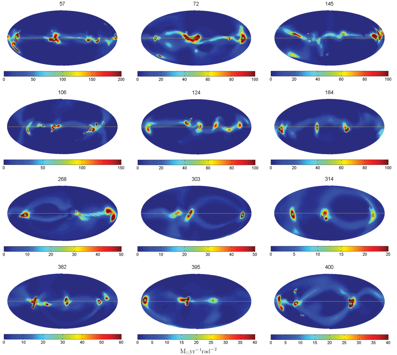
Figure 3. Coplanar inflowing streams and pancakes in a thick shell at (1-2)R_v . Shown as whole-sky Hammer–Aitoff maps of influx density are 12 different simulated galaxies in haloes of \sim 10^{12} M_\odot at z = 2.5 . They are selected to represent the many galaxies with at least three streams that almost perfectly lie on a great plane. The coordinates are rotated such that the best-fitting SP coincides with the equator. The colour represents radial influx of gas mass per solid angle. The centres of the three streams with the highest influx are marked by green dots. Typical flux densities in the streams are (50-150) M_\odot \text{ yr}^{-1} \text{ rad}^{-2} with the higher fluxes valid in the more massive haloes. Thin pancakes of \sim 10-15 M_\odot \text{ yr}^{-1} \text{ rad}^{-2} are seen between the streams, most frequently coinciding with the SP, but sometimes showing pancake segments that deviate from the SP.
