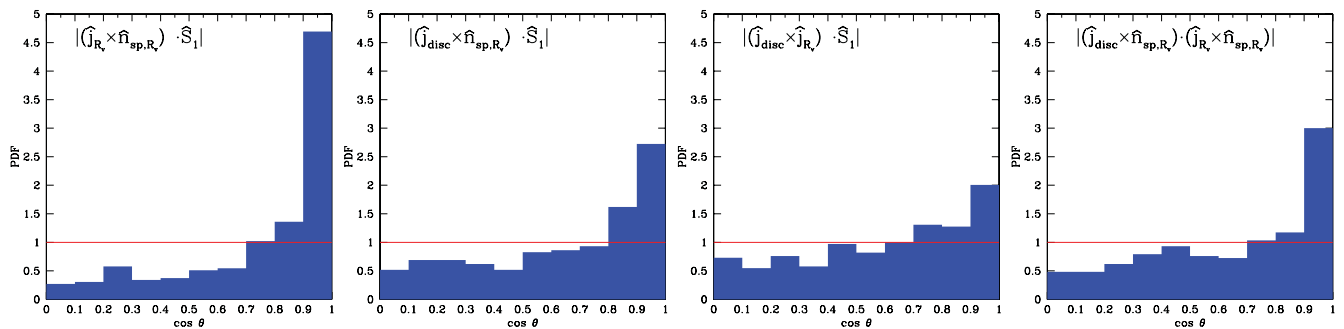
Figure 19. Alignment between the intersection of planes and the dominant stream: the AM at R_v ( \hat{J}_{R_v} ), the normal to the SP ( \hat{n}_{sp} ), the disc AM ( \hat{J}_{disc} ) and the vector along the dominant stream at R_v ( \hat{S}_1 ). The means are 0.76, 0.65, 0.60 and 0.71. The medians are 0.88, 0.73, 0.66 and 0.71. The KS p values are smaller than unity by many orders of magnitude in all cases.
