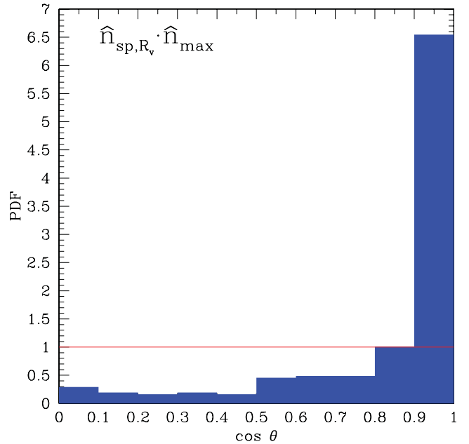
Figure B1. PDF of the cosine of the angle between the SP as defined in Section 3.1 and the maximum-influx plane. We see a strong alignment, with a median of \cos \theta = 0.96 .
