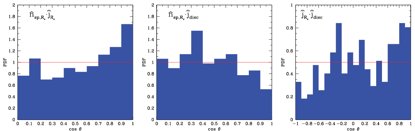
Figure 14. PDF of the cosine of the angle between pairs of planes. Left: the SP and the AM at R_v , with \langle \cos(\theta) \rangle = 0.56 , median = 0.60 and KS p = 0.001 . Middle: the SP at R_v and the disc AM, with \langle \cos(\theta) \rangle = 0.45 , median = 0.43 and KS p = 0.03 . Right: the AM at R_v and the disc AM, with \langle \cos(\theta) \rangle = 0.14 , median = 0.14 and KS p = 2 \times 10^{-4} . The AM at R_v is restricted to V_r < -0.5V_v . Note that \hat{n} , the normal to the SP, has no preferred orientation, so the associated range of cosine values is (0, 1) rather than (-1, 1) .
