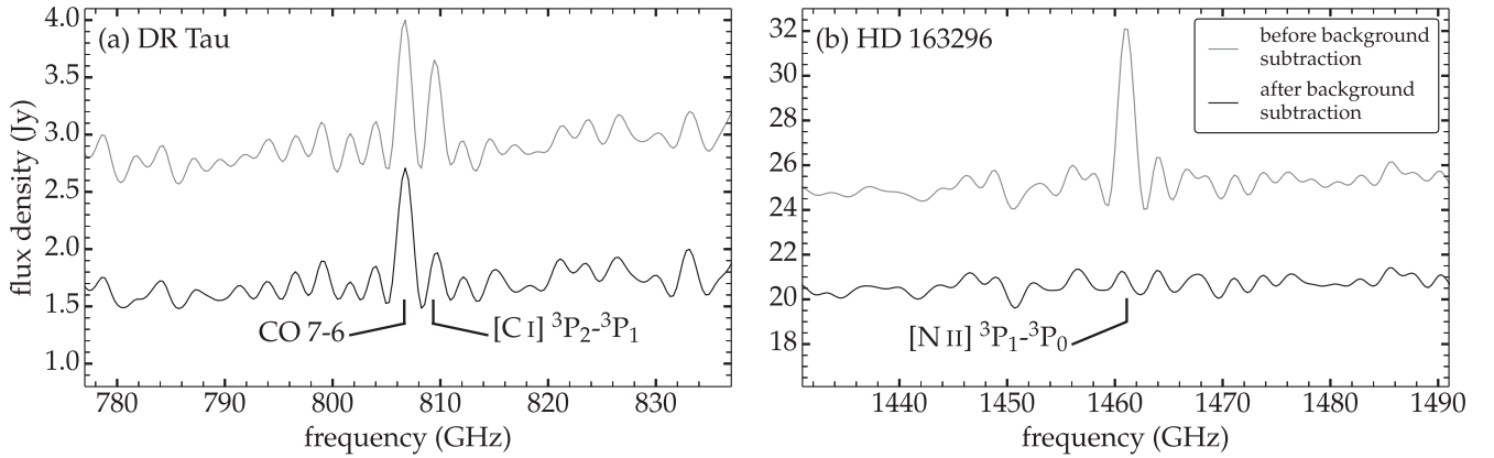
Figure 3. (a) Zoom of the 60 GHz section of the DR Tau spectrum centred around the CO 7–6 and [C I] ^3P_2-^3P_1 lines. The line of the neutral carbon atom coincides with the first sidelobe of the neighbouring CO line, but has significant flux of its own before background subtraction (grey), while its strength is reduced considerably after background subtraction is applied (black; same spectrum as in Fig. 2). (b) Zoom of the 60 GHz section of the HD 163296 spectrum centred around the [N II] line, again before and after background subtraction. This shows that the [N II] line towards HD 163296 originates from the extended background medium.
