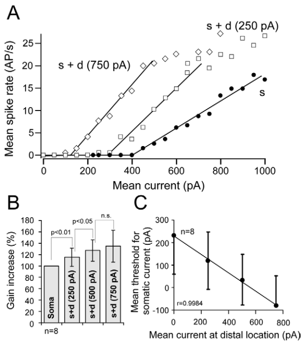
Figure 5. Modulation of the somatic current to rate transfer function by Gaussian current injection with constant mean into distal dendritic location. (A) Current to rate transfer function for somatic current injections in a particular neuron ( \sigma = 300 pA, \tau = 3 ms, \mu_{\text{start}} = 0 pA, \Delta\mu = 50 pA, step duration = 2 s, number of steps = 20), together with a noisy current injection into the dendrite with a fixed mean and standard deviation ( \mu_{\text{Dend}} = 0 pA, \sigma_{\text{Dend}} = 0 pA, filled circles; \mu_{\text{Dend}} = 250 pA, \sigma_{\text{Dend}} = 300 pA, open squares; and \mu_{\text{Dend}} = 750 pA, \sigma_{\text{Dend}} = 300 pA, open triangles). Note that with increasing mean current applied to the distal apical dendrite the f/I transfer function not only shifts to the left, but also the gain increases. The data points were fitted with a threshold-linear function (lines). (B) Summary from eight experiments illustrating the gain increase of the somatic transfer function in combination with distal currents of constant mean. (C) Mean threshold for somatic current injection versus constant mean current at distal location.
