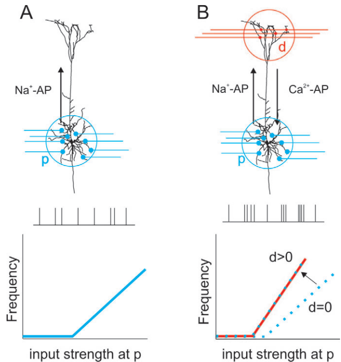
Figure 8. Dendritic gain modulation allows L5 pyramidal cells to associate spatially separated inputs. (A) Top panel; L5 pyramidal neuron with synaptic input to basal dendrite and soma only (p), generating the input–output relationship shown in the bottom panel. The firing pattern is nearly regular (spike train, middle). (B) Top panel; combination of proximal (p) and weak distal input (d) of constant mean strength shifts the threshold of the input–output relationship to a lower value (bottom panel), and at the same time increases its gain (arrow). This gain increase is the result of the interaction between the back-propagated AP ( \text{Na}^+ -AP) with the weak distal synaptic input, leading to forward propagated \text{Ca}^{2+} -AP, which in turn evokes an AP burst at the axonal spike initiation zone. Hence, the association of spatially segregated inputs leads to an increase in the gain and could be signaled to the postsynaptic neuron by the presence of bursts.
