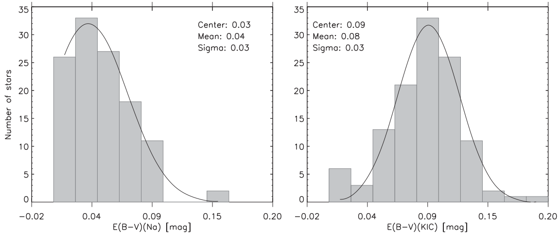
Figure 1. Distributions of E(B - V)(\text{Na}) (left-hand panel) and E(B - V)(\text{KIC}) (right-hand panel). Gaussian fits are shown by solid lines. Central values, arithmetic means and standard deviations of both distributions are indicated in figures.
