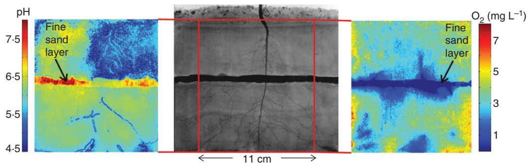
FIG. 3. Container with white lupin in a quartz sand captured by NR (corrected raw images, centre), and the same container through fluorescence O_2 -sensitive foil (right) and pH-sensitive foil (left).
