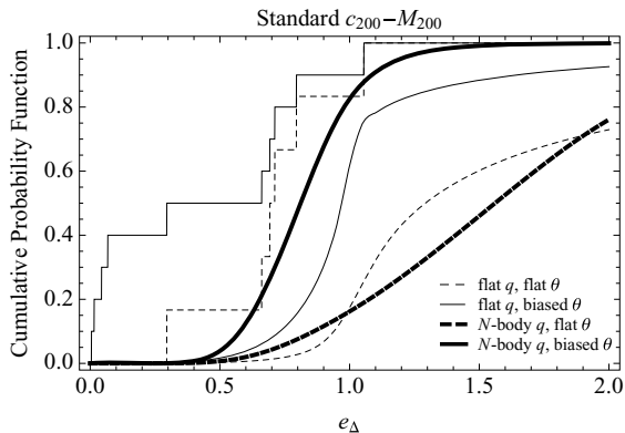
Figure 2. Predicted cumulative distribution functions for elongation versus measurements. The full and dashed step-lines are for the full observed sample and for the clusters with e_\Delta > 0.1 , respectively; the smooth functions are the predicted distributions under different assumptions (see legends). The left- and right-hand panels show the observed elongations computed assuming either a standard or an enhanced mass–concentration relation, respectively.
