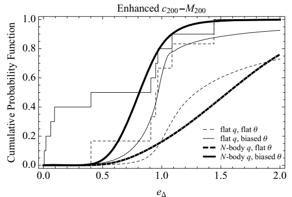
Figure 2. Predicted cumulative distribution functions for elongation versus measurements. The full and dashed step-lines are for the full observed sample and for the clusters with e_\Delta > 0.1 , respectively; the smooth functions are the predicted distributions under different assumptions (see legends). The left- and right-hand panels show the observed elongations computed assuming either a standard or an enhanced mass–concentration relation, respectively.
