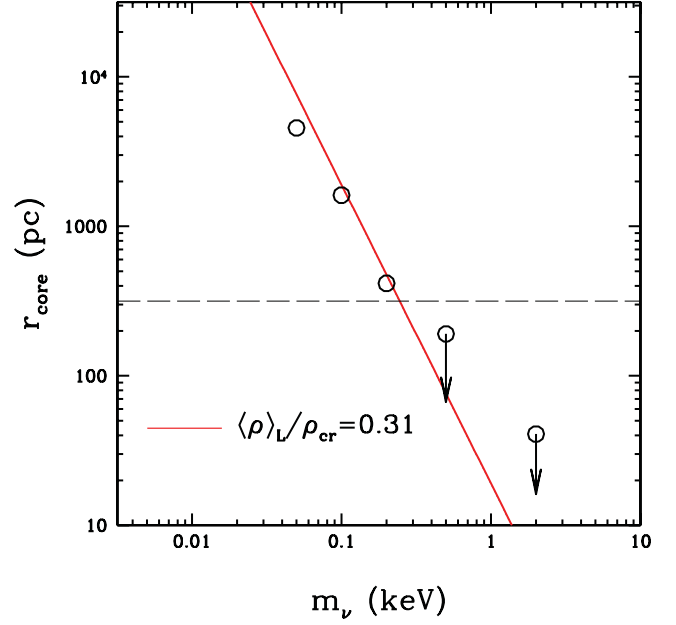
Figure 7. Comparison between core size in simulations (open symbols) and the theoretical expectation for an M = 10^{12} M_\odot halo (solid line). The dashed line is the gravitational softening of our simulations. All points below this line should be considered as upper limits on the core size.
